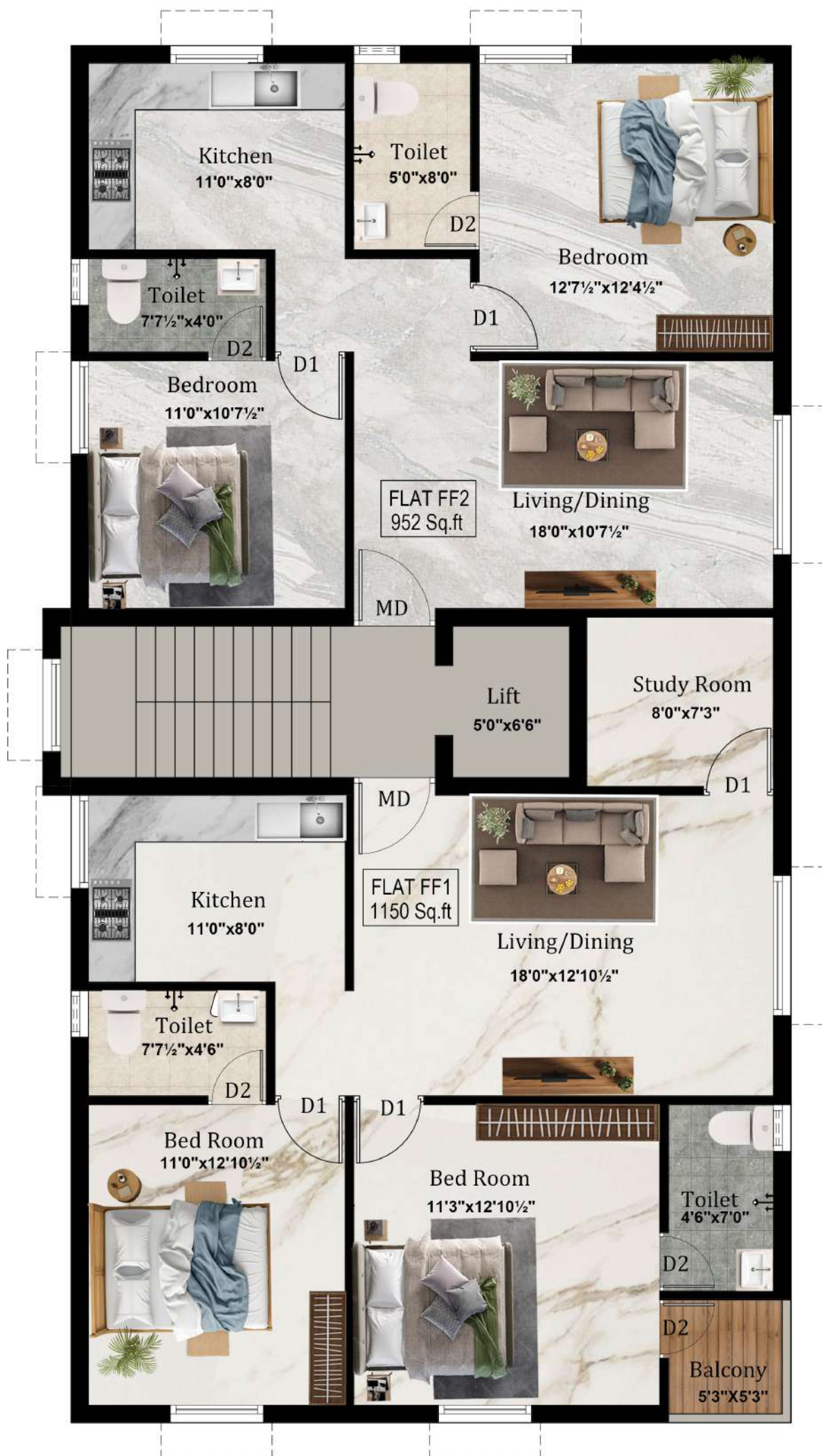
TYPICAL FLOOR PLAN BLOCK - A FIRST TO THIRD
